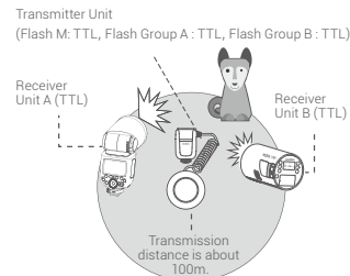
Auto Flash Shooting with Two Receiver Units
